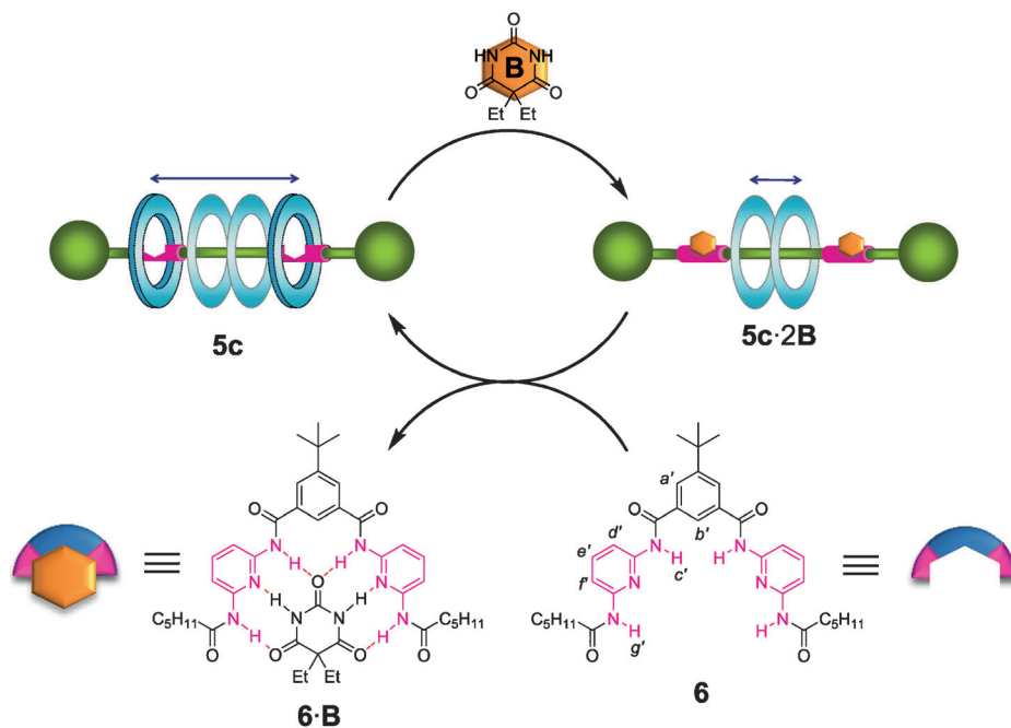
Scheme 3. Reversible control of the amplitude of the translational motion in the interlocked bis(di(acylamino)pyridine) 5c by the formation of a stronger ADA-DAD array.
